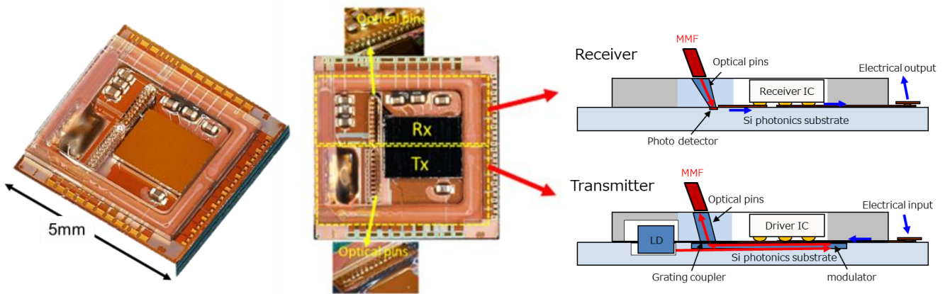
Structure of Optical I/O Core
